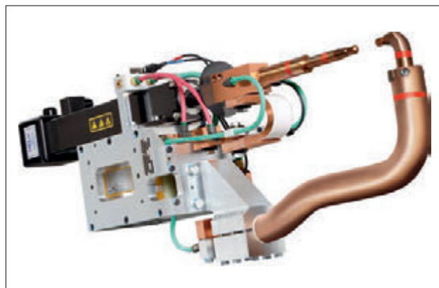
Global Gun Generation 3 (C-Type)
