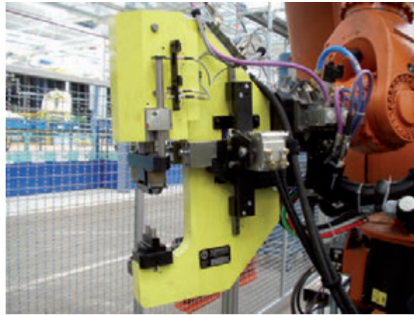
Adapter plate flanged to the back or base for connection to automation robots or quick-change systems
