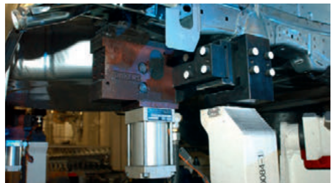
Underbody clamp with fitted and positioned floor assembly
