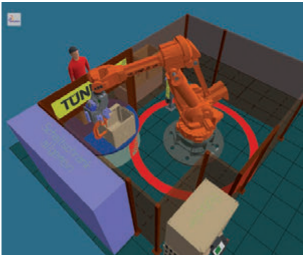
Robot cell for spot welding operations on stainless steel tank
