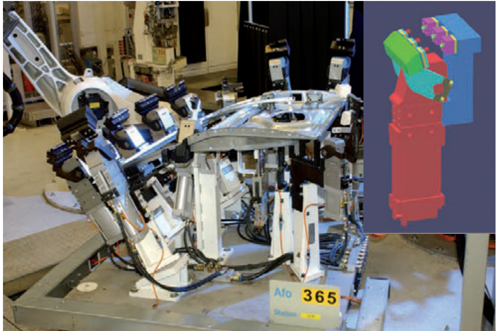
Fixture with power press units for stamping of naps/beads into steel sheets
