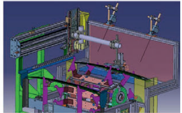
Detail view of the handling system for component removal and transfer to the robots
