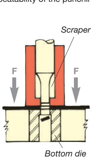
Polyurethane retainer of high-strength wear-free plastics
