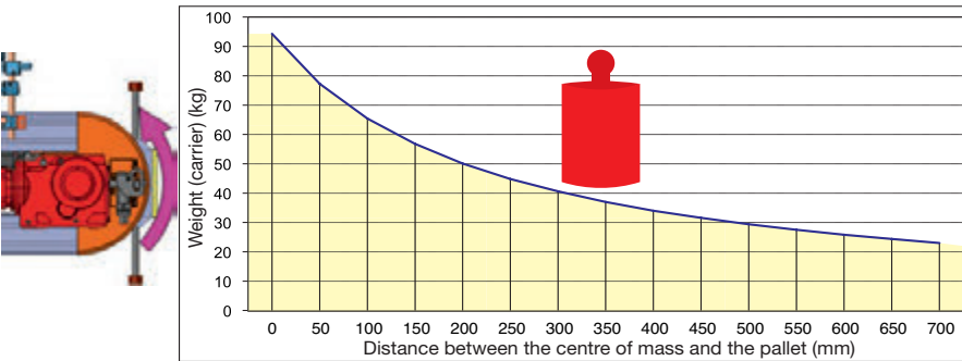
Maximum load of the component carrier as a function of the pallet spacing
