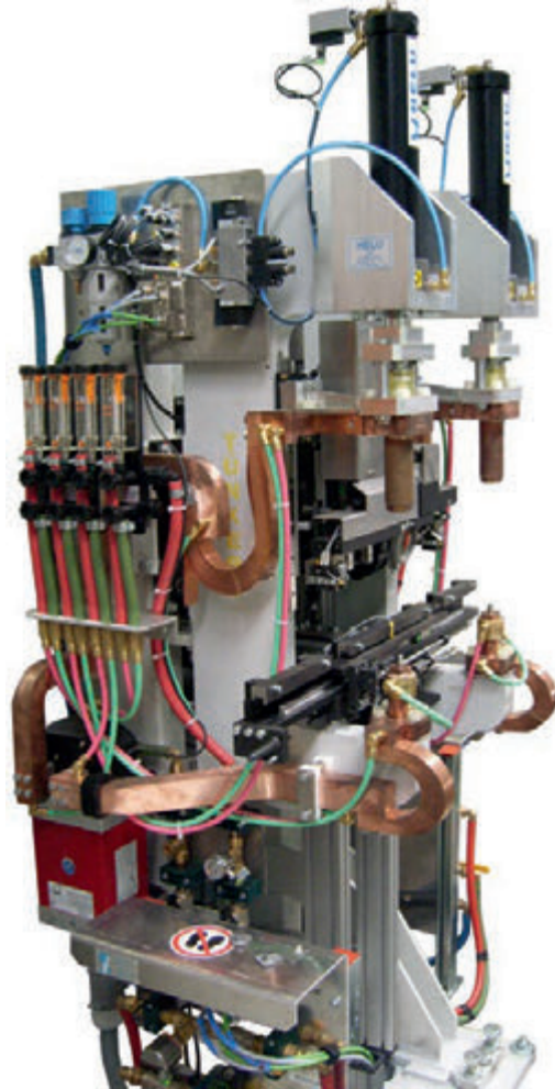
Dual C-frame weld unit
