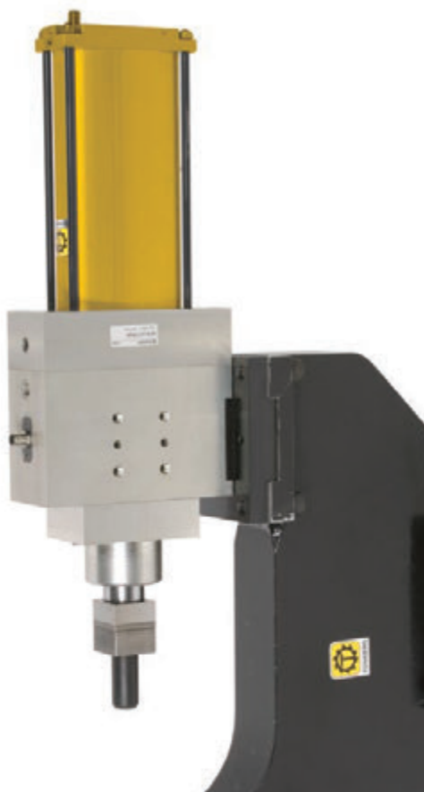
MZ 80 with piston rod guide, 25 kN, 100 mm stroke, for hole punching operations
