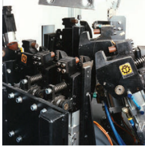
Compact unit with pneumatic drive
