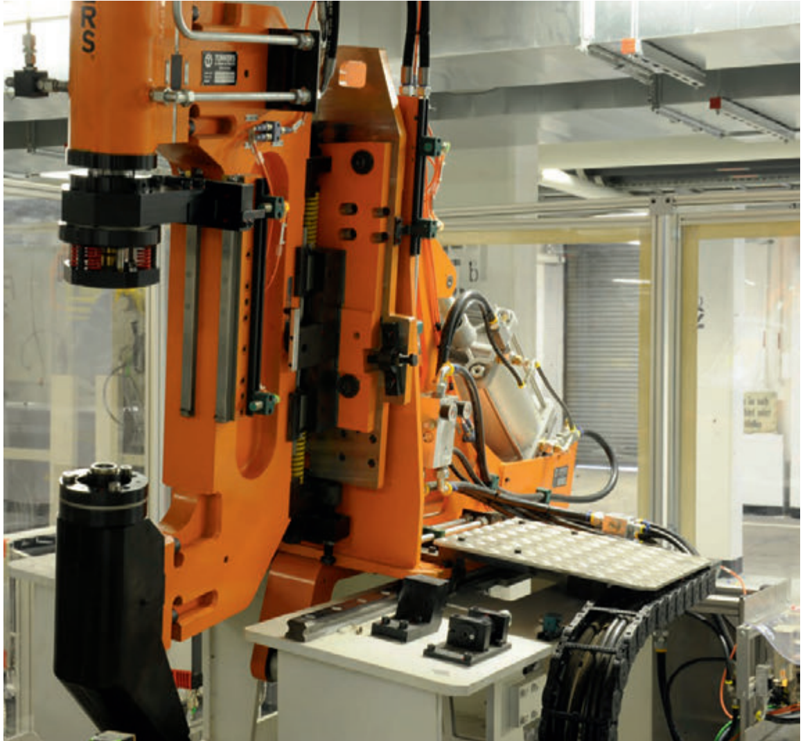
Stationary C-Frame unit
