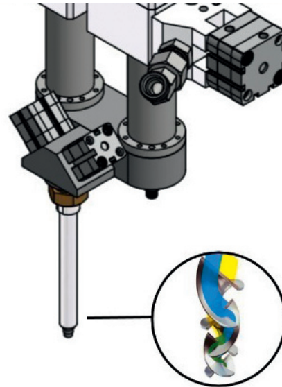
2K Static Mixer
