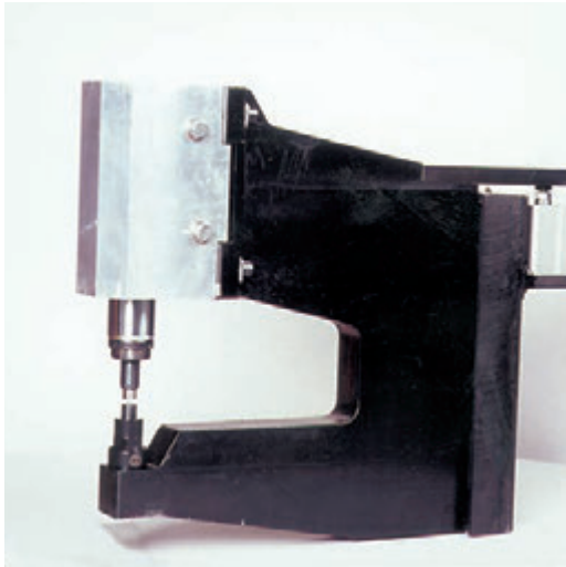
Hydraulic C-frame system for joining applications with hydraulic drive
