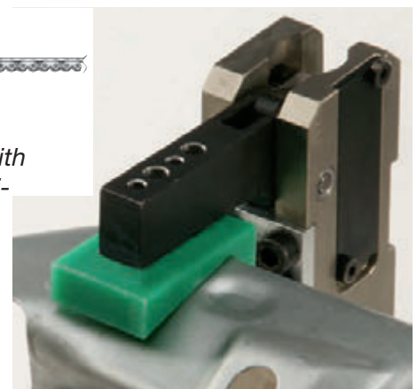
Clamping sheet metal components
