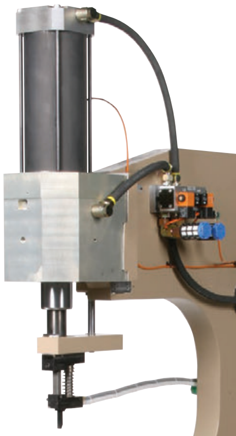
MZ 100 with piston rod guide, 60 kN, 150 mm stroke, for nut piercing operations
