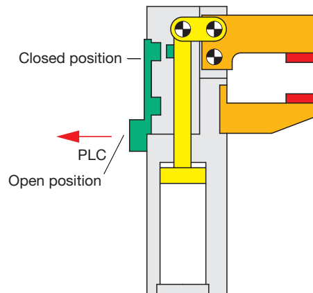
Position sensing cassette fitted to a knee-lever clamp
