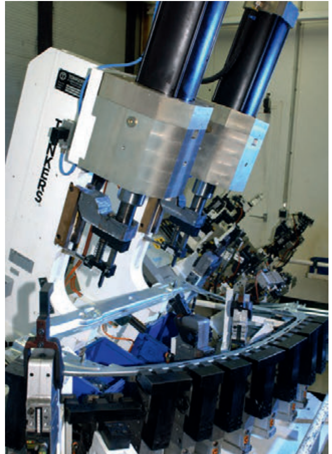
Set device for knobs embossing and nuts piercing
