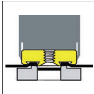
Setting of Nuts
