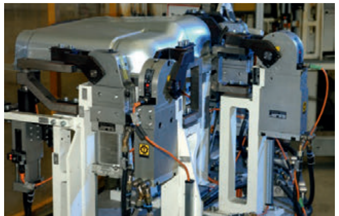
Group of clamps with Vario and Alpha Clamps
