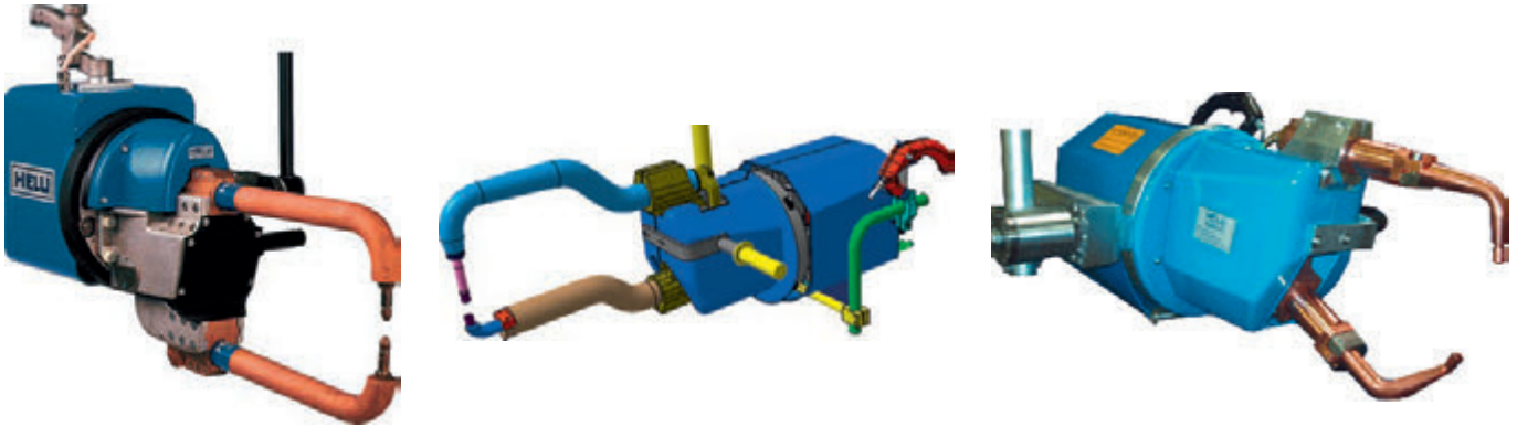
Standard transformer manual weld guns
