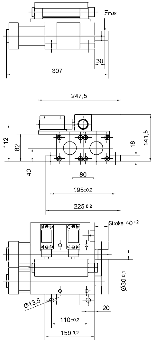
Dowel toggle switch T01S Dowel synchronisation switch T03S
