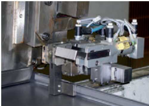
PKS 25 pneumatic clamp used as a component end stop in a welding fixture – domestic appliance manufacture
