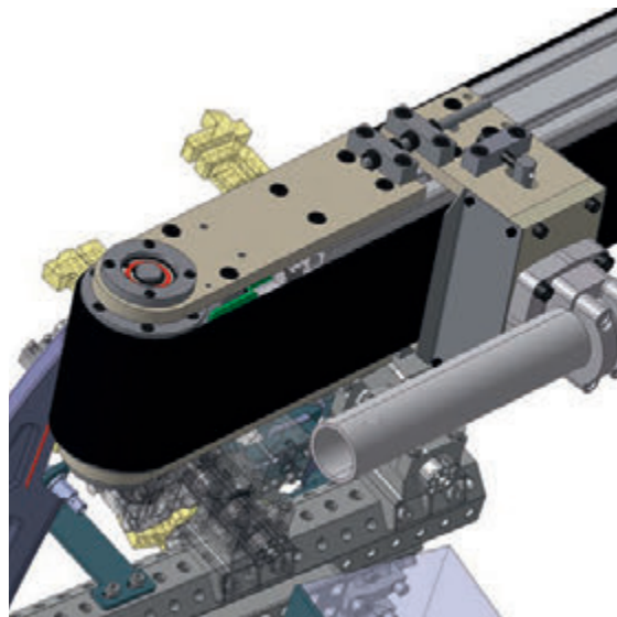
Detail view of the belt tensioning device
