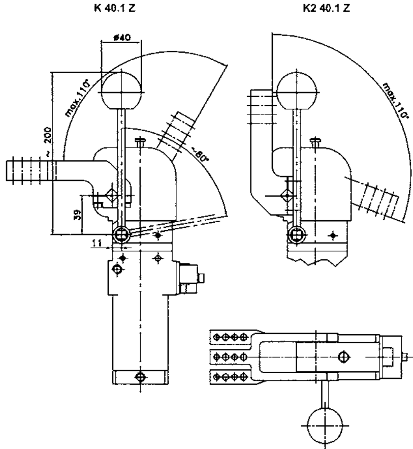
Hand lever supplied unattached
