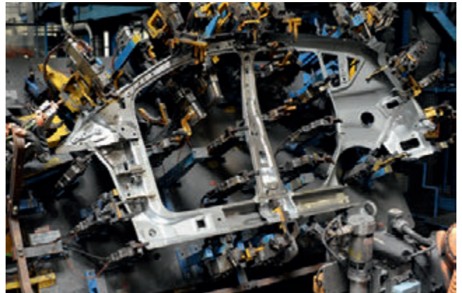
Clamping fixture with Vario Clamp for side wall body panel
