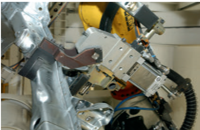
Vario Clamp for positioning side members
