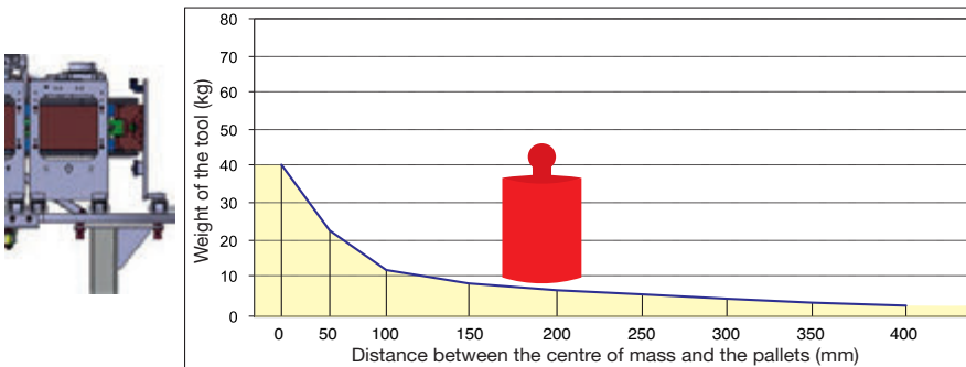
Maximum load of the carrier and the component as a function of the pallet spacing
