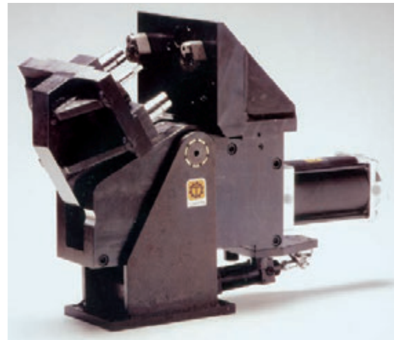
Hydraulic multiple punch tool with toggle-lever clamp
