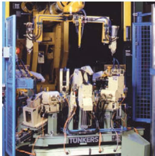
Turnkey joining station with C-frames and power press unit
