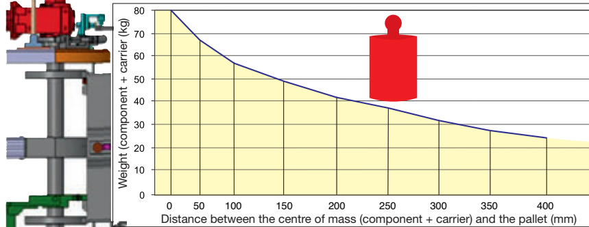
Maximum load as a function of the pallet spacing
