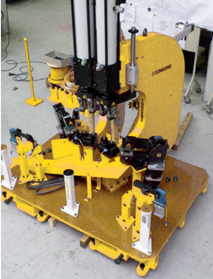
Fixture for bolt punching and cutting of the component "door"
