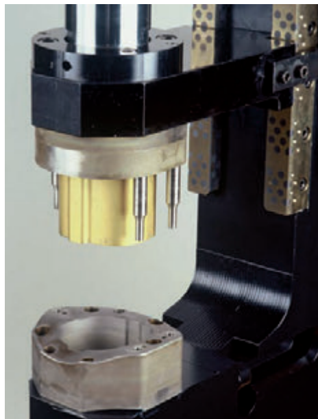
Bulkhead punch unit, right-hand drive breach
