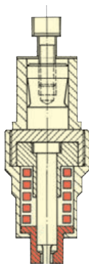
Tool cartridge with integrated stamp holder and spring-loaded retainer
