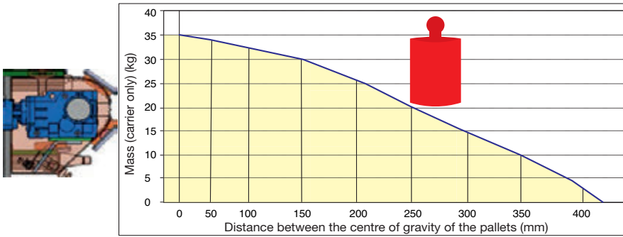
Maximum load of the component carrier as a function of the pallet spacing
