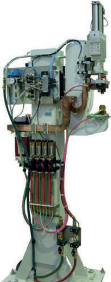
Single C-frame weld unit
