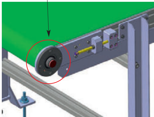
Detail view of the belt tensioning device
