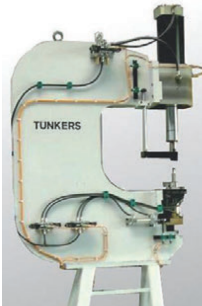
C-frame mounted to pedestal for stationary applications with customer specific base frame
