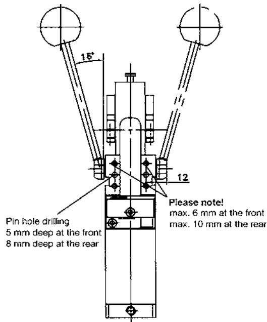
Hand lever supplied unattached
