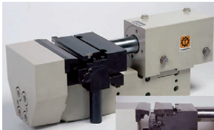
C-frame system for folding short sheet metal offcuts, with integral hold-down device
