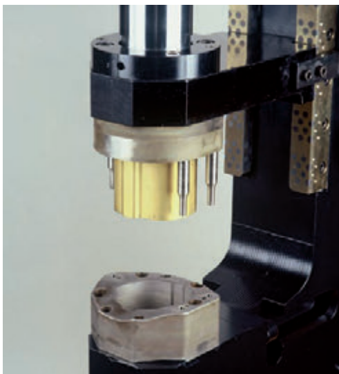
Horizontal or vertical clamp adjustment, ensures that process forces cannot affect the workpiece directly during forming and cause deformation. Alternatively spring-loaded or pneumatically controlled.
