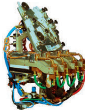
Special weld gun (AEG)
