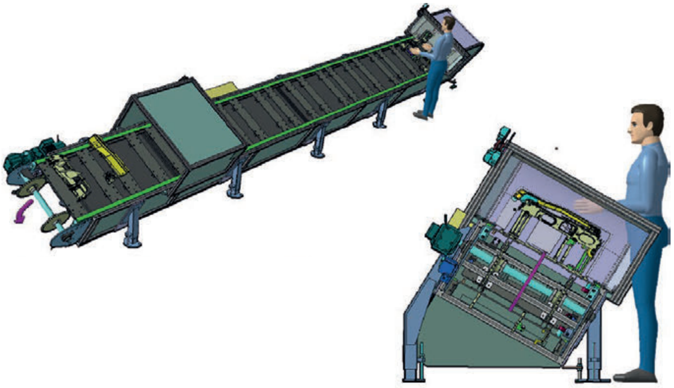
Chain conveyor in ergonomic inclined position
