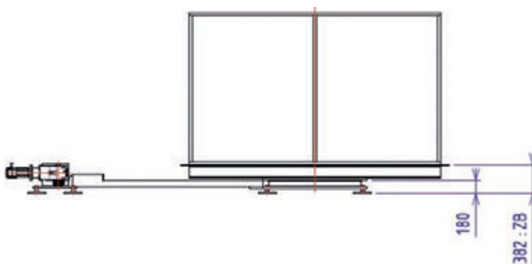
SOPAP TXR 1100 with basic framework and external motor mounting
