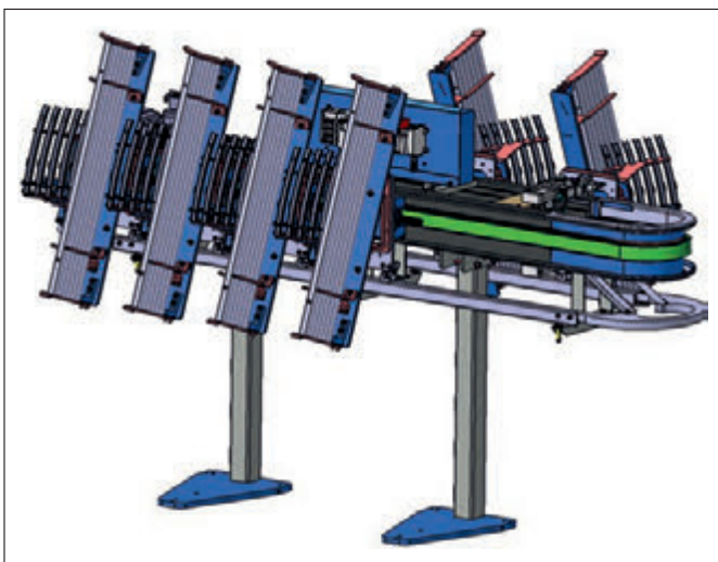
LFS 90° conveyor with pallets arranged transversely
