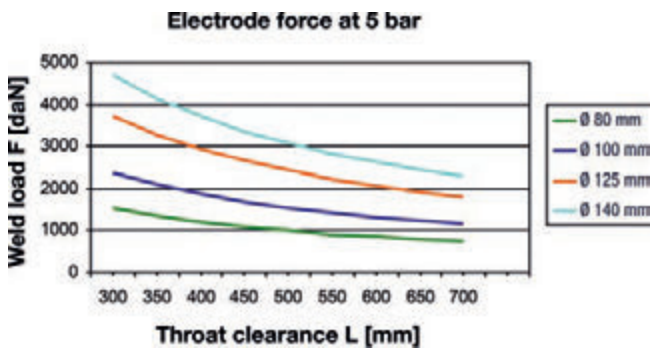
HD transformer weld guns
