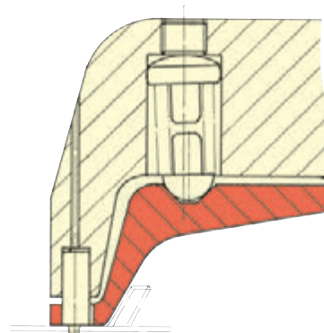
Special retainer in forked or pin-form design, adjusted to the interference situation
